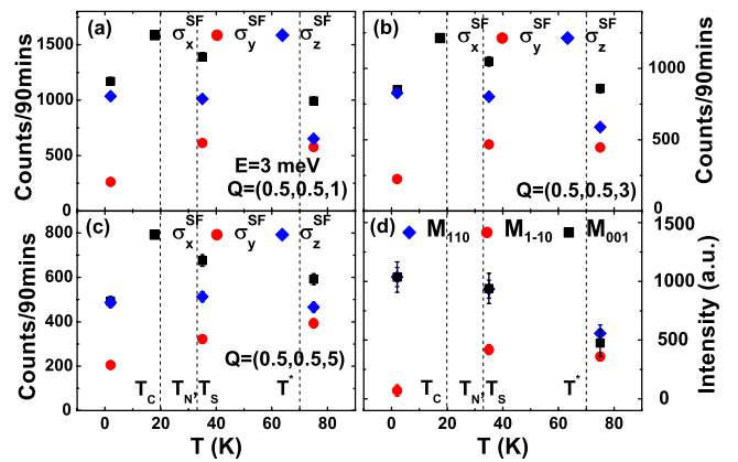
FIG. 5 (color online). (a)–(c) Temperature dependence of neutron SF scattering cross section \sigma_{x,y,z}^{\text{SF}} at 3 meV and \mathbf{Q}_{1,2,3} = (0.5, 0.5, L) with L = 1, 3, 5 . (d) The temperature dependence of magnetic response along the [110] ( M_{110} ), [1\bar{1}0] ( M_{1\bar{1}0} ), and [001] ( M_{001} ) directions. Clear in-plane anisotropy persists up to T^* = 70 K.
