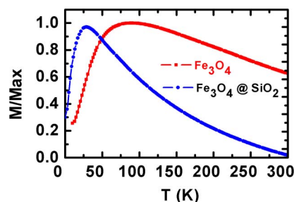
Figure 2 | Temperature-dependent zero-field-cooled (ZFC) magnetization of the as-prepared \text{Fe}_3\text{O}_4 and \text{Fe}_3\text{O}_4/\text{SiO}_2 nanoparticles.
