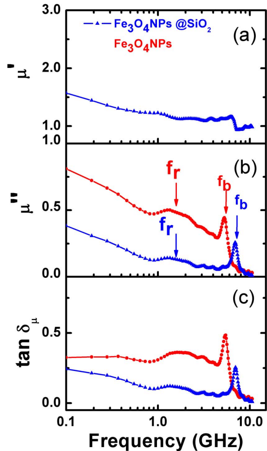
Figure 4 | (a) Frequency dependence of real part \mu' ; (b) imaginary part \mu'' and (c) magnetic loss tangent \tan \delta_\mu = \mu''/\mu' of the \text{Fe}_3\text{O}_4/\text{paraffin wax} and \text{Fe}_3\text{O}_4/\text{SiO}_2/\text{paraffin wax} .
