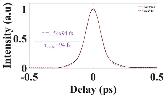
Fig. 7. Typical intensity autocorrelation trace for idler at 1670 nm: the solid trace is experimental data, and the red dot curve is the corresponding hyperbolic secant shape fitting.
