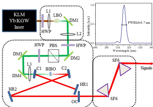
Fig. 1. Sketch for the experimental setup of the femtosecond OPO based on a BIBO. HWP: half wave plate; DM1–DM4: dichroic mirrors; PBS: polarization beamsplitter; L1–L3: lenses; HR1–HR2: high-reflectivity flat mirrors; OC: output coupler; C1 and C2: concave mirrors; SF6: prism. Inset: optical spectrum of the SHG pulses.
