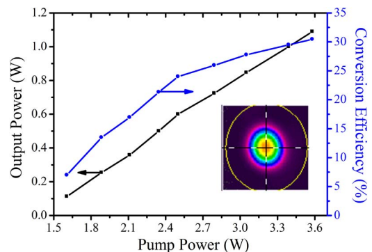
Fig. 2. Output power (black) and the corresponding conversion efficiency (blue) of the femtosecond OPO based on BIBO. Inset: beam profile at the maximum output power.
