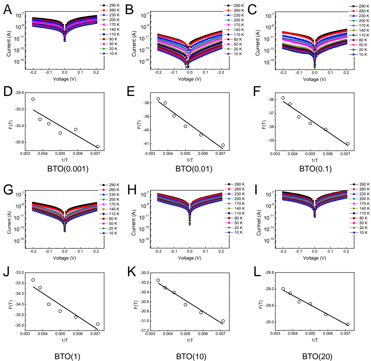
Figure S18, related to Figure 5. I - V curves (A-C, G-I) and F(T) - 1/T plots (D-F, J-L) of the corresponding I - V data measured for Pt/BTO(0.001)/SNT0 to Pt/BTO(20)/SNT0 junctions at HRS at different temperatures, where the lines fit the F(T) - 1/T curves in (D-F, J-L).
