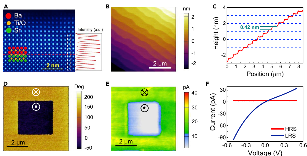
Figure 1. Geometry and Ferroelectric Properties of 7 u.c.-Thick BaTiO 3 (BTO) Film Deposited on Nb-doped SrTiO 3 (SNT0) Substrate
