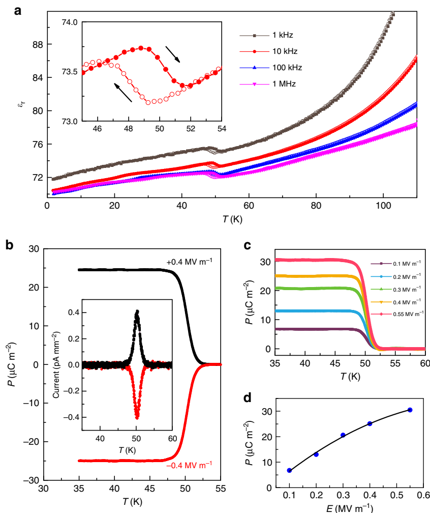
Fig. 5 Spin-induced ferroelectricity in the binary perovskite \text{Mn}_2\text{O}_3 . a The dielectric constant as a function of temperature. A dielectric peak with a hysteresis is seen at T_2 = 49 K, indicating a first-order ferroelectric transition. No apparent dielectric anomaly at T_1 = 101 K is detected. The inset shows an enlarged view around T_2 . b The electric polarization as a function of temperature measured with a poling electric field of 0.4 \text{ MV m}^{-1} . The polarization is reversed by a negative poling field. The inset presents the pyroelectric current as a function of temperature after subtracting the background. The peak around T_2 confirms spin-induced ferroelectricity. c The electric polarization measured with different poling electric field. d The electric polarization as a function of poling electric field
